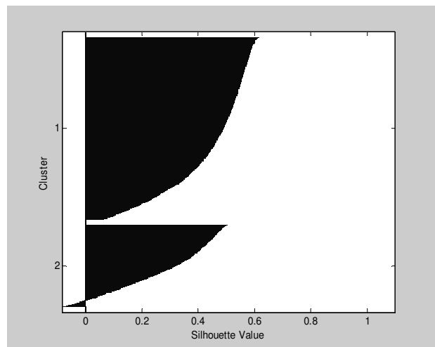
Figure 1. Silhouette plot with 2 clusters for hearing aid type of right ear air conduction frequencies.
